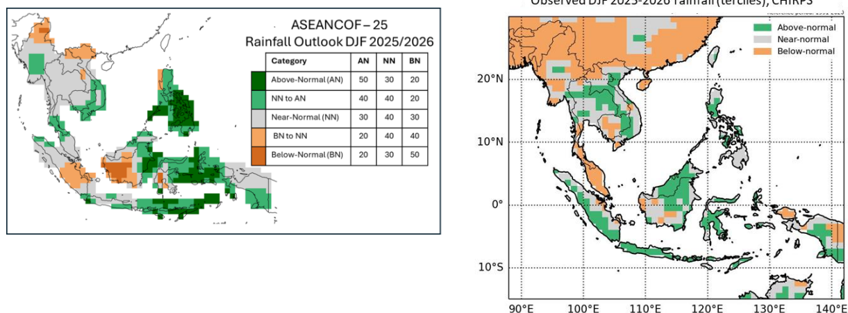
Figure E1: DJF 2025/2026 ASEANCOF outlook (left) observed DJF rainfall in terciles (right, climatology 1991-2020). The rainfall dataset is CHIRPS (Funk et al. 2014).
