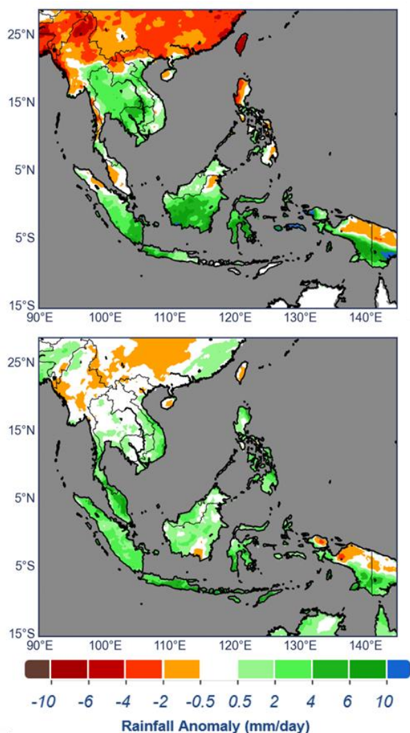
Figure 6: Rainfall anomaly (in mm/day) for July – September 2022 (upper) and October – December 2022 (lower) against 1991-2020 climatology from CHIRPS dataset. Areas in green experienced wetter than average conditions, while those in orange experienced drier than average conditions. Data: IRI Data Library .
