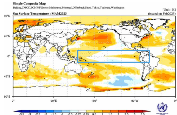
Figure 10: SST anomaly prediction for March-May (MAM) 2023 from WMO showing ENSO neutral conditions in the tropical Pacific Ocean (blue box). Credit: WMO Lead Centre for Long-Range Forecasting.
