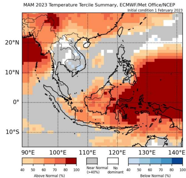
Figure 13: Temperature tercile summary predictions from the multi-model ensemble forecast for March-May (MAM) 2023. Red shades show regions with a higher likelihood of warmer conditions, while blue shades show regions with a higher likelihood of cooler conditions (contains modified Copernicus C3S information).
