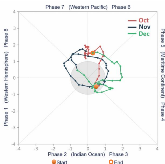
Figure 8: MJO strength and phases during October (red), November (blue) and December (green) 2022. The orange dots mark the start and end of the timeseries. Data: BoM, Australia .
