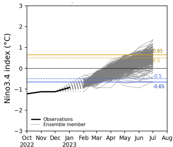
Figure 9: Nino3.4 detrended SST anomaly predictions from the modified C3S Copernicus models output showing colder temperatures until the end of February. Subsequently, most models predict ENSO neutral conditions for March-May (MAM) 2023 period.
