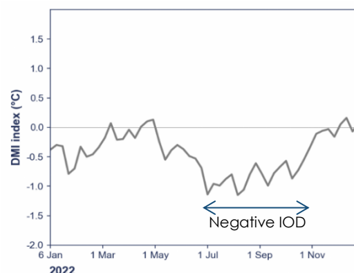
Figure 3: Indian Ocean Dipole (IOD) index showing an episode of negative IOD event in the second half of 2022. Data Credit: Bureau of Meteorology, Australia.
