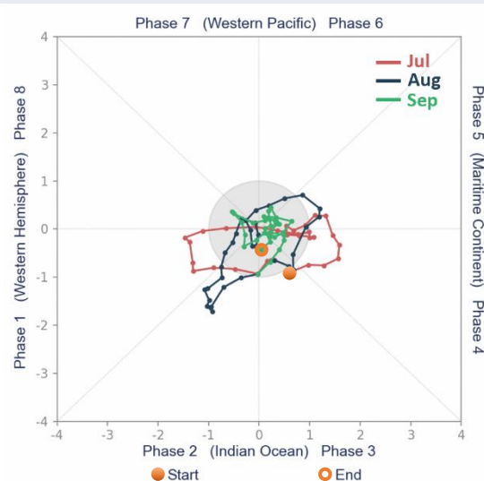
Figure 7: MJO strength and phases during July (red), August (blue) and September (green) 2022. The orange dots mark the start and end of the timeseries. Data: BoM, Australia .
