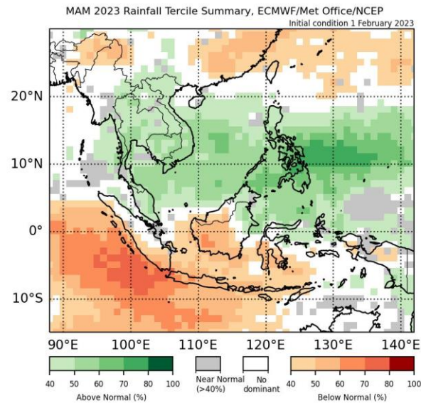
Figure 12. Rainfall tercile summary predictions from the multi-model ensemble forecast for March-May (MAM) 2023. Brown shades show regions with a higher likelihood of drier conditions, while green shades show regions with a higher likelihood of wetter conditions (contains modified Copernicus C3S information).
