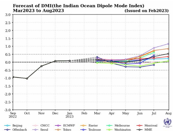
Figure 11: IOD index predictions, from models available on the WMO Lead Centre for Long-Range Forecasting, show neutral IOD conditions in the tropical Indian Ocean during March-May 2023 period. Credit: WMO Lead Centre for Long-Range Forecasting.
