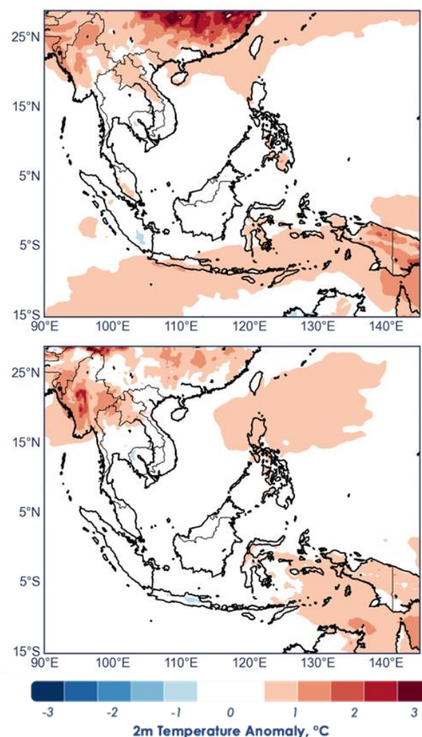
Figure 5: Average 2-metre temperature anomalies (°C) against 1991-2020 climatology for July – September 2022 (upper) and October – December 2022 (lower) show a mix of near- to above-average temperatures (white and red shades, respectively) for Southeast Asia in the second half of 2022. Data: ECMWF .
