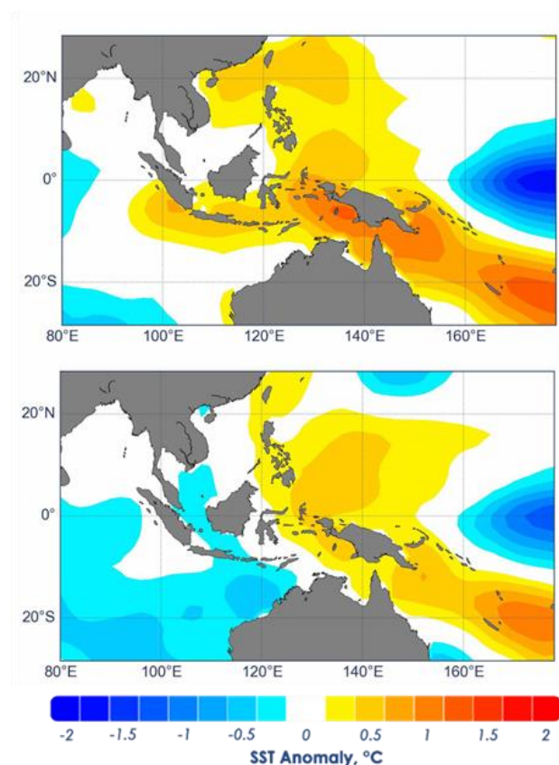
Figure 4: Average sea surface temperature (SST) anomalies for July – September 2022 (upper) and October – December 2022 (lower). SSTs were warmer than average for much of the Southeast Asia region in July – September 2022 with the warm pattern sustaining over the eastern region in October – December 2022. The reference climatology is from 1991 to 2020. Data: IRI Data Library .
