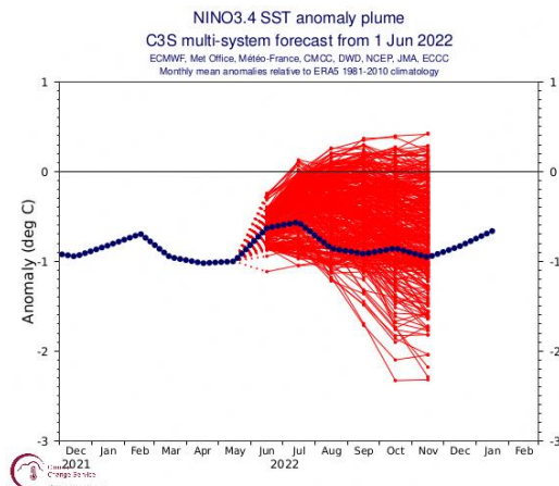
Figure 2: Forecasts of Nino3.4 index's strength (red lines) in June 2022 for the second half of 2022 from various seasonal prediction models of international climate centres. Observed values are in blue. Credit: Copernicus C3S.C
