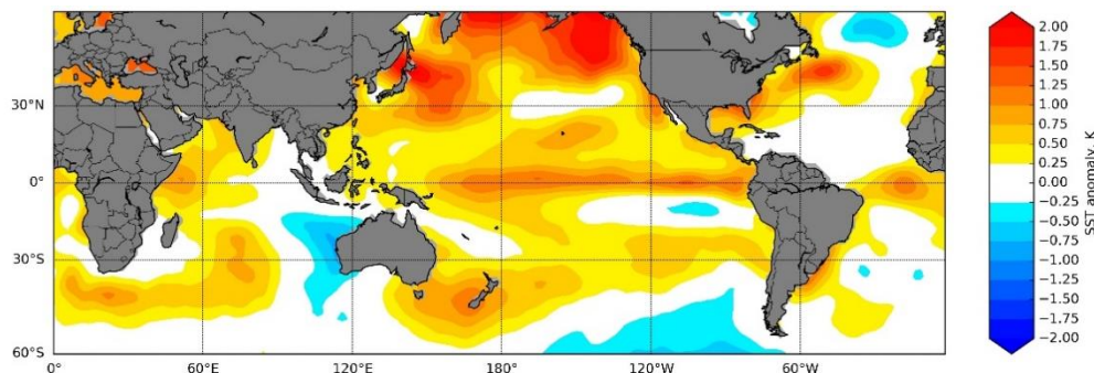
Figure 3: Warmer-than-average sea-surface temperature anomalies (warm shades) for October-December 2018 season over the tropical Pacific Ocean neared El Niño thresholds. However, the atmosphere failed to respond and to impact the global weather patterns. Data: ERSST version 5.
