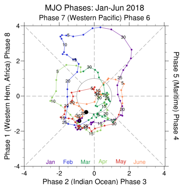
Figure 5: MJO phases from January to June 2018. The MJO was very strong and active from around mid-January to mid-February 2018. Data: BoM, Australia.
