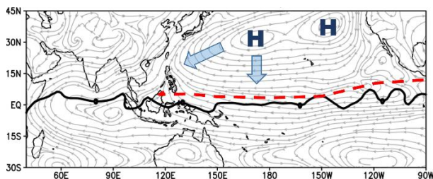
Figure 30. Low-level winds at 850 hPa (grey streamlines) and the subtropical high (H) associated with the subsidence of the Hadley cell located over the Pacific Ocean and the absolute vorticity at 925 hPa (solid black line). The ITCZ was positioned near equator (dashed red line). Credit: NCEP/CPC CDAS.
