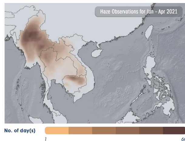
Figure 11. Haze areas for January – April 2021. Smoke haze from clusters of hotspots were observed particularly in Cambodia and the northern parts of the Mekong sub-region.
