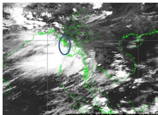
Figure 27. Himawari-8 satellite image at 0920 UTC, 16 June 2021 shows rain clouds over the Rakhine Coast of Myanmar (blue circle). Credit: Japan Meteorological Agency.
