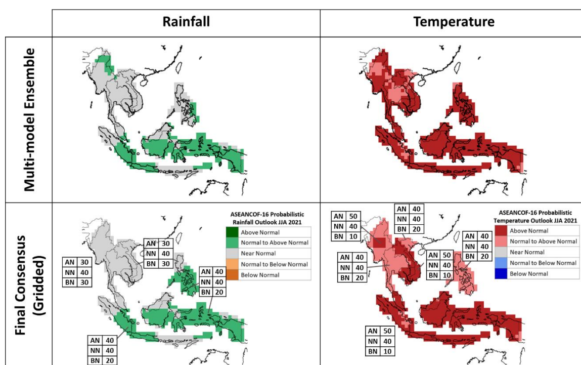
Figure 43. Multi-model ensemble (top) was used as a basis for the final consensus outlook for June – August 2021 (bottom).
