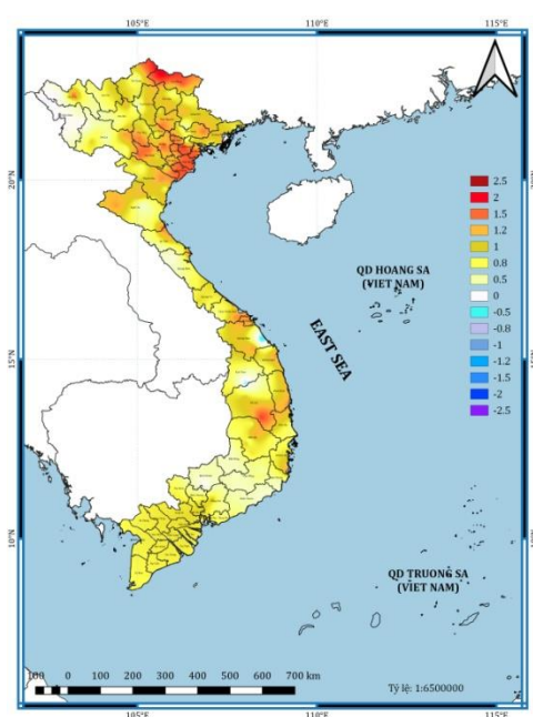
Figure 20. Temperature anomaly over Viet Nam in June 2021.
