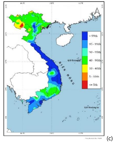
Figure 20: Total rainfall amount, anomaly, and percentile (from a to c) over Viet Nam during the period 31 March 2022 to 2 April 2022.
