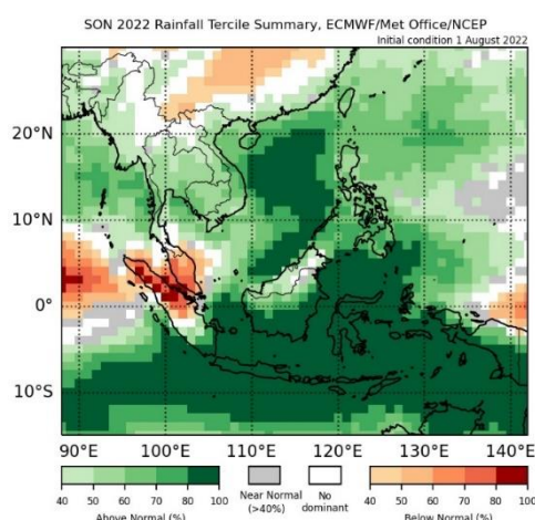
Figure 16. Rainfall tercile summary predictions from multi-model ensemble for SON 2022, showing regions with a higher likelihood of drier conditions (brown) and wetter conditions (green).
