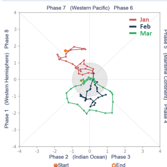
Figure 5. MJO strength and phases during January (red), February (blue), and March (green) 2022. The orange dots mark the start and end of the timeseries. Data: Bureau of Meteorology, Australia .
