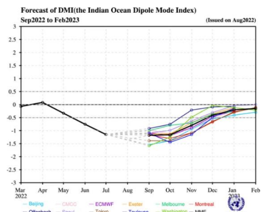
Figure 15. IOD index predictions, from models available on the WMO Lead Centre for Long-Range Forecasting, continue to be negative but will rapidly weaken towards the end of the year. Credit: WMO Lead Centre for LRF .
