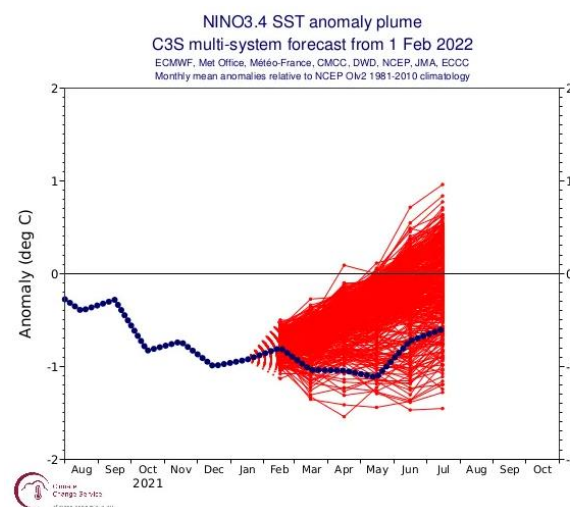
Figure 2. Prediction of Nino3.4 index's strength (red lines) from February 2022 from various seasonal prediction models of international climate centres. Observed values are in blue. Credit: Copernicus C3S.
