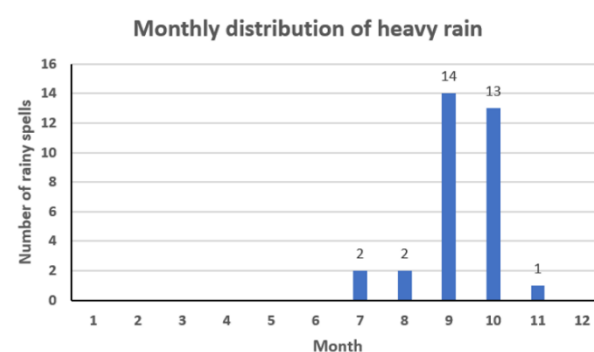
Figure 18: Monthly distribution of heavy rain over Central Viet Nam.
