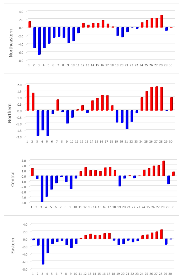
Figure 38: Time series of the anomaly of minimum temperature during 1 – 30 April 2022 across various parts of Thailand (climatological period of 1991 – 2020). Credit: TMD weather stations.
