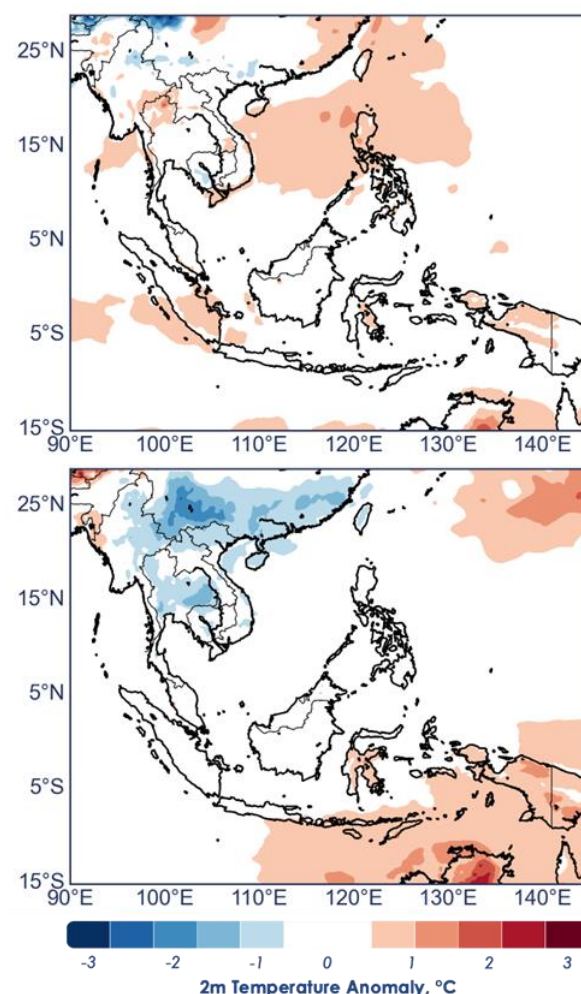
Figure 7. Average 2-metre temperature anomalies (°C) against 1991 – 2020 climatology for January – March 2022 (upper) and April – June 2022 (lower) shows warmer conditions (red shades), near-average conditions (white), and cooler conditions (blue shades) for Southeast Asia in the first half of 2022. Data: ECMWF .
