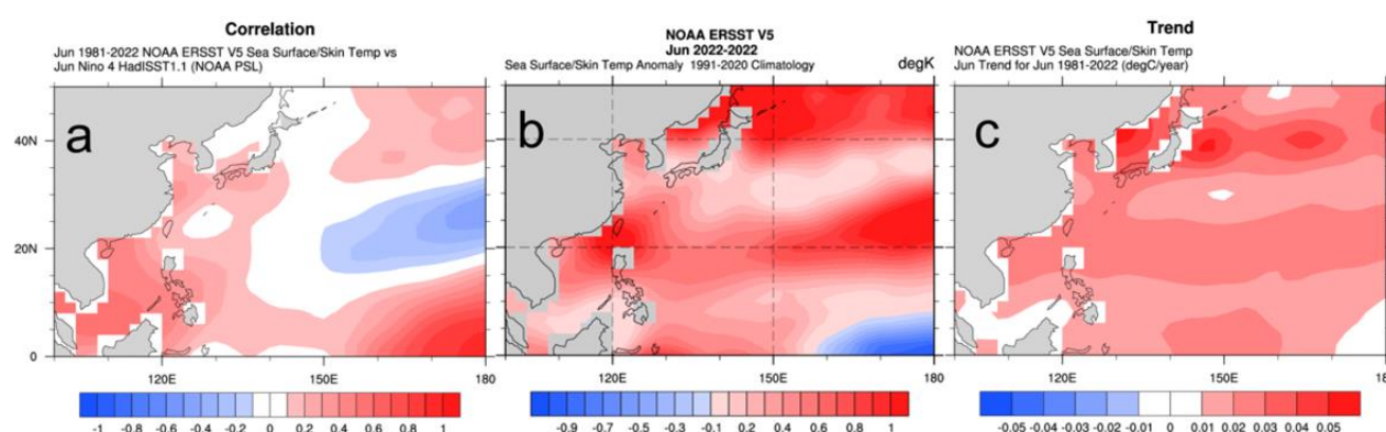
Figure 28: Relationship of SST and large-scale environment: (a) spatial correlation of Niño 4 and SST during June from 1981 to 2022, (b) SST anomalies in June 2022, and (c) trend from 1981 to 2022 in the Western North Pacific. Credit: WRIT, 2022.
