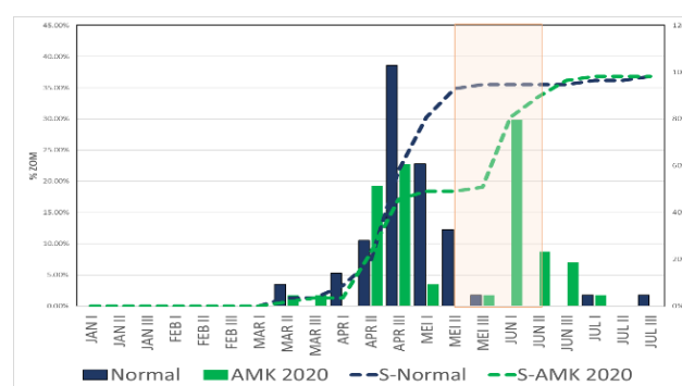
Figure 19: The percentages of “Zona Musim” or ZOM (areas that have clear distinctions between the wet and dry seasons) for the “Awal Musim Kemarau” or AMK 2020 (onset of the dry season) represented by green bars, compared to normal represented by dark blue bars. The corresponding accumulated percentages (right-axis) of AMK 2020 are shown by the green dotted lines, compared to the normal shown by the blue dotted lines.
