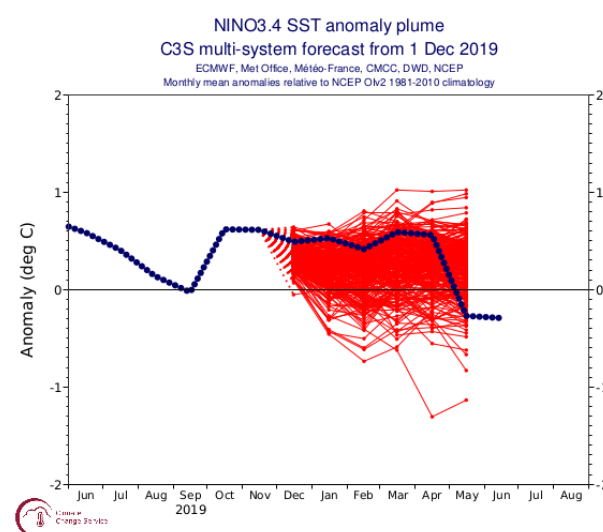
Figure 2: Forecasts of Nino3.4 index's strength (red lines) in December 2019 for the first half of 2020 from various seasonal prediction models of international climate centres. Observed values are in blue. Credit: Copernicus C3S.
