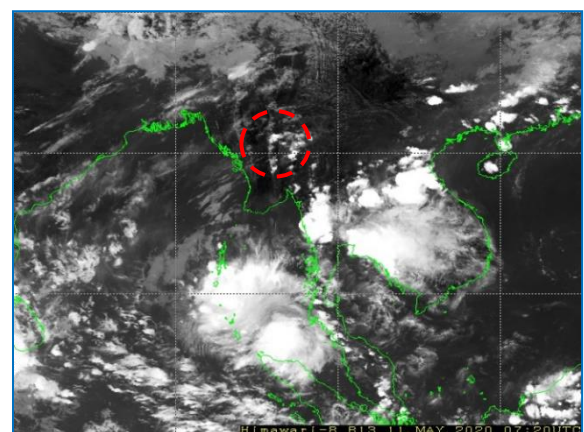
Figure 28: Himawari-8 Satellite image on 11 May 2020 at 0720 UTC showing heavy-rain clouds over Central Myanmar (red circle). Credit: Japan Meteorological Agency.
