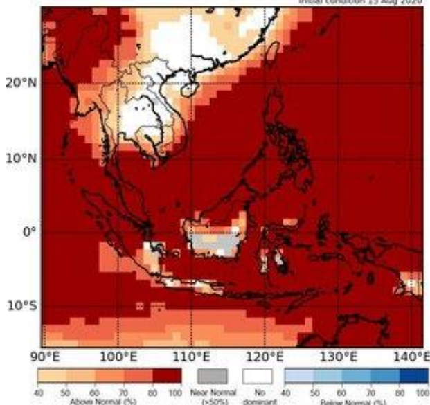
Figure 15: Temperature tercile summary predictions of multi-model ensemble model for September-November (SON) 2020. Red (blue) shades show regions with a higher likelihood of warmer (cooler) conditions (contains modified Copernicus C3S information).
