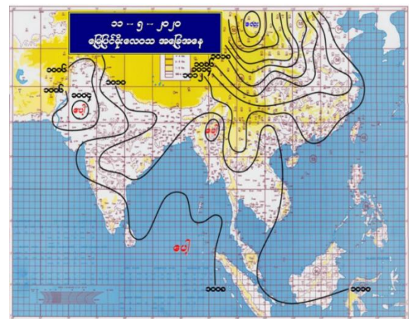
Figure 27: Surface weather chart by the DMH on 11 May 2020 (00 UTC) showing a low-pressure area over the Mandalay Region.
