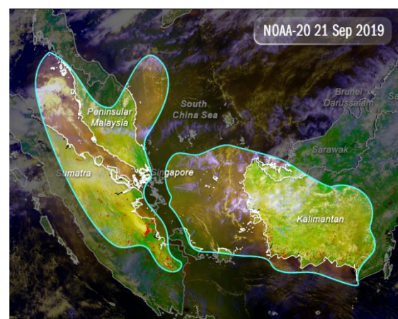
Figure 10: NOAA-20 satellite image on 21 September 2019 shows transboundary smoke haze (highlighted areas) affecting Malaysia and Singapore blown in from fires in Sumatra and Kalimantan by the prevailing winds.
