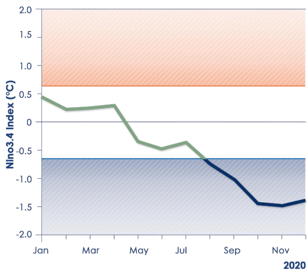
Figure 1: The Nino3.4 index (detrended) using 1-month SST anomalies. Warm anomalies ( \geq +0.65 ; orange) correspond to El Niño conditions while cold anomalies ( \leq -0.65 ; blue) correspond to La Niña conditions, otherwise: neutral ( > -0.65 and < +0.65 ). Reference methodology: Turkington et al., 2018.
