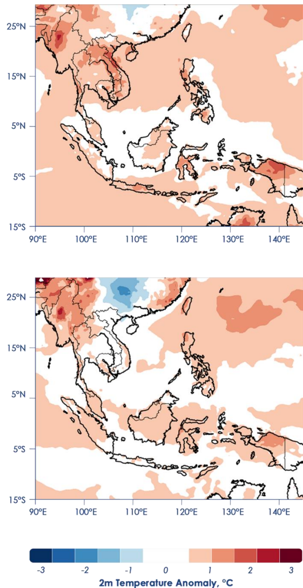
Figure 5: The average 2-metre temperature anomalies (against 1981 – 2010 climatology) for July – September 2020 (top) and October – December 2020 (bottom) show a mix of near to above average temperatures (red and white, respectively) for Southeast Asia in the second half of 2020. Data: ECMWF.
