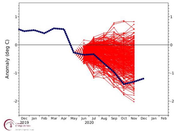
Figure 2: Forecasts of Nino3.4 index's strength (red lines) in June 2020 for the second half of 2020 from various seasonal prediction models from international climate centres. Observed values are in blue. Credit: Copernicus C3S.
