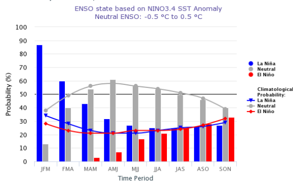
Figure 9: ENSO probabilistic forecast based on the Nino.3.4 index which shows a higher likelihood of neutral conditions (grey) occurring from the March-May (MAM) 2018 season onwards. Credit: IRI/CPC.
