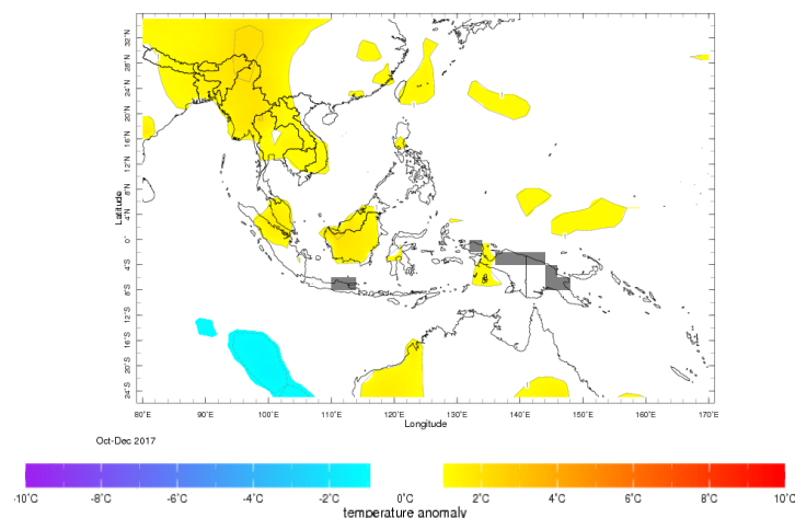
Figure 4: October-December 2017 seasonal average surface temperature anomaly (°C) showing warmer conditions over mainland Southeast Asia and central parts of the Maritime Continent (Kalimantan, Peninsular Malaysia, and central-north Sumatra). Credit: IRI Maproom.
