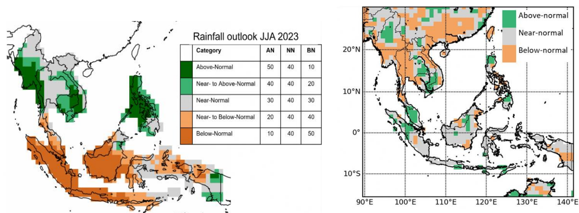
Figure D1: JJA 2023 ASEANCOF outlook (left) observed JJA rainfall in terciles (right, climatology 1991-2020). The rainfall dataset is CHIRPS (Funk et al 2014).
