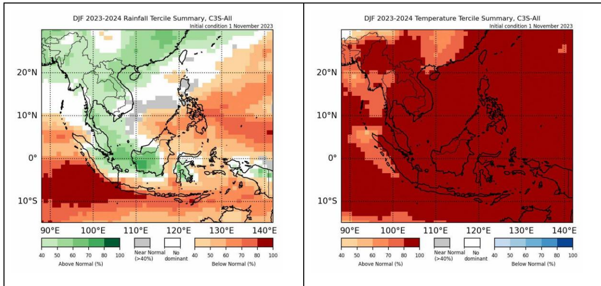
Figure B1: Outlook from the C3S seasonal models for DJF 2023/2024 for rainfall (left) and temperature (right). The models used included NCEP, ECMWF, JMA, UK Met Office, DWD, CMCC and MeteoFrance.
