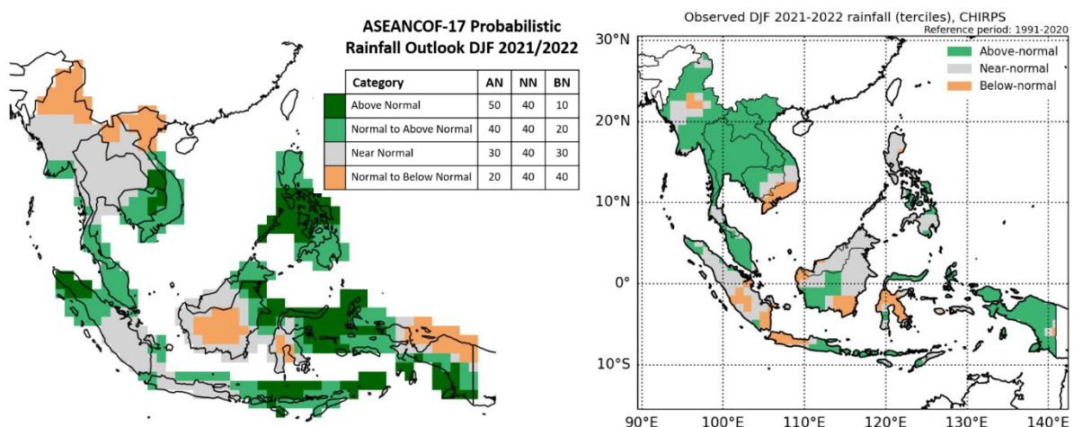
Figure C1: DJF 2021/2022 ASEANCOF outlook (left) observed DJF rainfall in terciles (right, climatology 1991-2020). The rainfall dataset is CHIRPS (Funk et al 2014).
