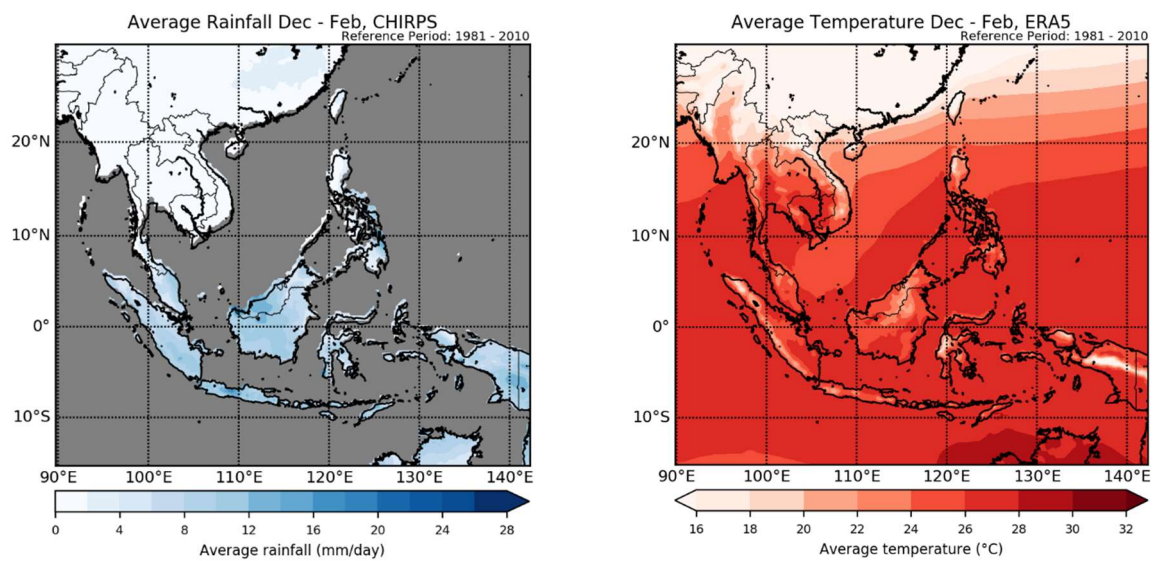
Figure A1: Mean rainfall (left, CHIRPS) and mean temperature (right, ERA5) for DJF for the climatology period 1981-2010.
